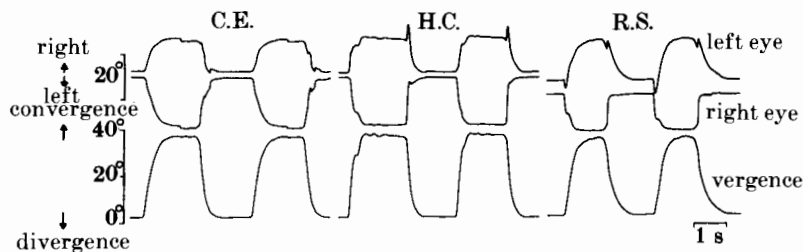
FIGURE 2. Representative eye movements of the three subjects (C. E., H. C. and R. S.) when they shifted gaze between LEDs A and E, both of which were located along each subject's median plane (see figure 1 for their relative distances from the subject). Viewing, as well as eye-movement recording, was binocular.
