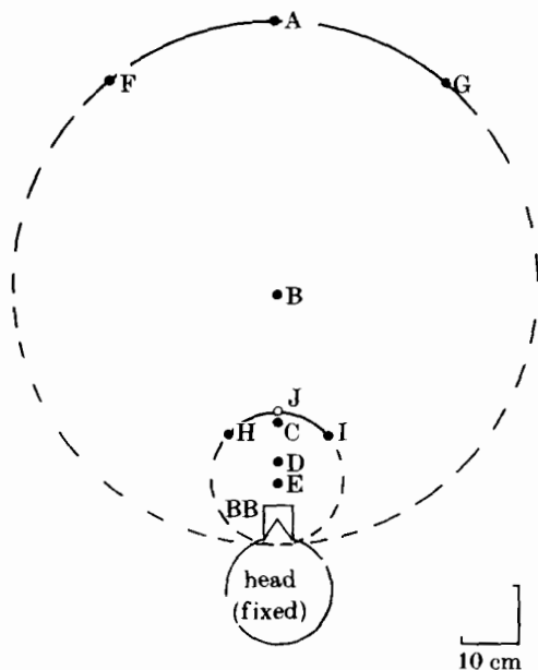
FIGURE 1. Top view of the subject and the arrangement of the LED targets, drawn to scale. The subject's head was supported by a bite-board (BB). The LEDs are shown by solid dots. The significance of their placement and the particular pairs lighted in each experiment are described in the text.
