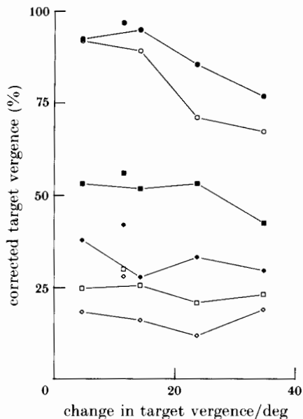
FIGURE 12. Percentage of change in target vergence corrected by ocular vergence when target pairs were viewed monocularly. The solid symbols signify viewing by the right eye and the open symbols signify viewing by the left eye. Subject C.E. is shown by circles, H.C. by squares, and R.S. by diamonds. The connected symbols represent the responses to the targets in the median plane; the single symbols refer to the asymmetric targets (change in target vergence 11^\circ ). The percentage of correction includes corrections made by both saccadic and smooth vergence responses.
