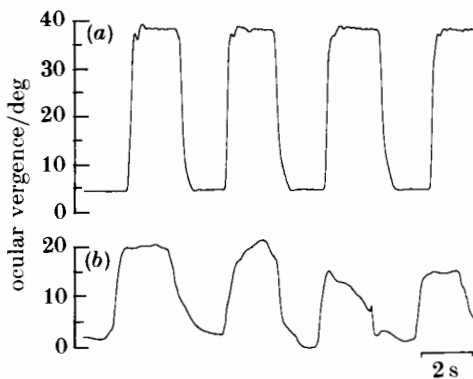
FIGURE 14. Ocular vergence responses of subject H.C. (a) when he shifted gaze between LEDs A and E visible along his median plane and (b) when he shifted gaze between imagined LEDs at the same locations while in complete darkness.
