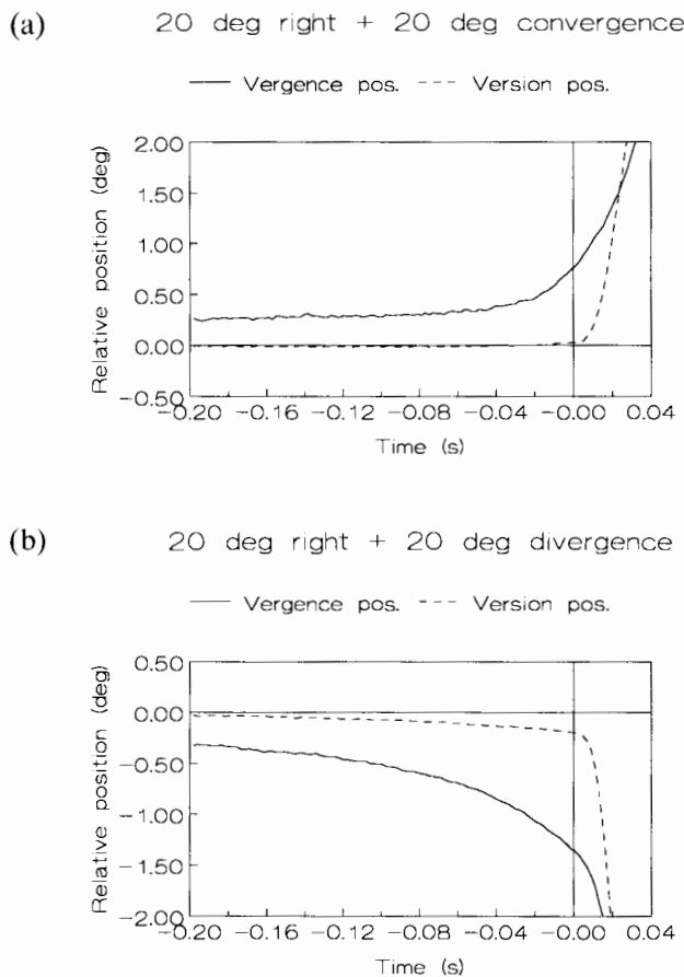
FIGURE 13. Details of pre-saccadic vergence and version angles for convergent (a) and divergent (b) gaze-shifts involving shifts of 20 deg in both vergence and version (subject: AP). This stimulus configuration was chosen for illustration because it elicits, on average (see Fig. 12), substantial (though not extreme) pre-saccadic vergence movements in the direction appropriate for the imminent gaze-shift. Saccadic onset (version velocity >15 deg/sec) is at t = 0 . Positions have been shifted to fit the high-resolution scale; thus, the numbers on the ordinate do not represent absolute angles.
