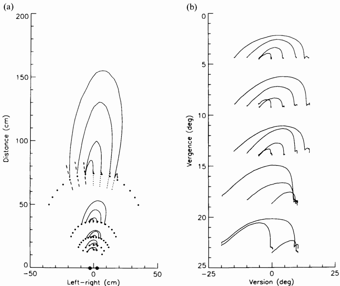
FIGURE 7. Typical trajectories of conjugate saccades (5–30 deg) at different iso-vergence angles (5–25 deg). Rightward saccades of subject AP are shown. (a) Trajectories, plotted in metric coordinates (as in Fig. 6). (b) Same set of saccades, plotted in angular coordinates (vergence vs version angles). Notice that, due to the geometric relations (see Fig. 1) the outward loops of conjugate saccades decrease strongly in amplitude for increasing iso-vergence (a), even though the absolute magnitude of transient divergence increases at the same time (b).
