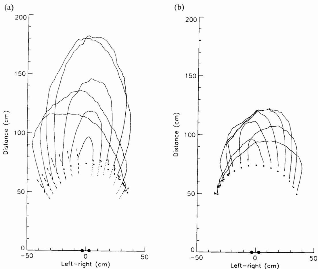
FIGURE 6. Typical trajectories of the binocular fixation point during conjugate saccades (10–70 deg) at 5 deg iso-vergence, projected on the horizontal plane of regard, seen from above. Rightward (a) and leftward (b) saccades of subject CE are shown; the difference in sizes of the loops in the two directions is idiosyncratic, and at the same time marks the overall range that we observed in our subjects. Dots on the X -axis represent positions of the eyes. Iso-direction lines are drawn through the starting (dashed lines) and end positions (dotted lines) of the trajectories.
