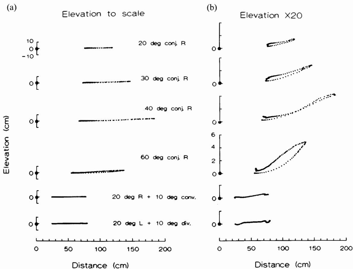
FIGURE 9. Projections of gaze-trajectories (subject: CE) on the sagittal plane, viewed from the right side, to illustrate that vertical components of horizontal gaze-shifts were very small. (a) Vertical and horizontal movements plotted on equal scales.
